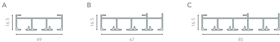
A. 3 track channel side view B. 4 track channel side view C. 5 track channel side view
